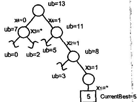
Figure 2: Execution of Max_Abs for Example 4
