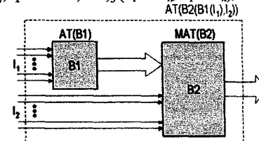
Figure 1: MAT in Composition of ATs
